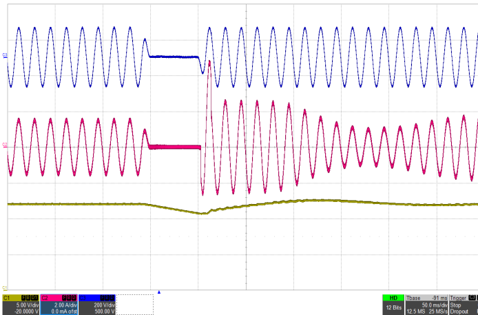
Figure 9: Line drop out with 400µF hold-up capacitor at full load current (115Vrms, 60Hz) Top: Vin (200V/div), Mid: Iin (2A/div), Bottom: Vout (5V/div), Timebase: (50ms/div).
