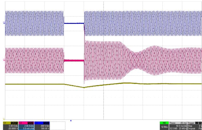
Figure 10: Line drop out with 400µF hold-up capacitor at full load current (115Vrms, 400Hz) Top: Vin (200V/div), Mid: Iin (2A/div), Bottom: Vout (5V/div), Timebase: (50ms/div).
