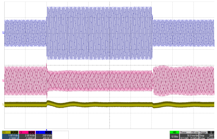
Figure 16: Input voltage transient response with 200µF hold-up capacitor at full load current (115Vrms-230Vrms-115Vrms, 400Hz), Top: Vin (200V/div), Mid: In (2A/div), Bottom: Vout (1V/div), Timebase: (50ms/div).
