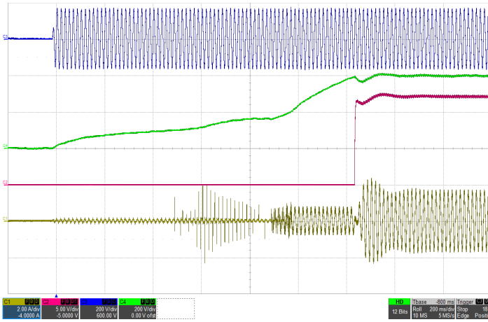
Figure 13: Typical startup waveform with 200µF hold-up capacitor (115Vrms, 60Hz) Top: Vin (200V/div), Top Middle: Hold-up capacitor voltage (200V/div), Bottom Middle: Vout (5V/div), Bottom: In (2A/div), Timebase: (200ms/div).
