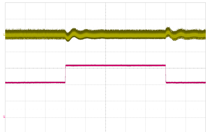
Figure 12: Regulated model output voltage response to step-change in load current with 200µF hold-up capacitor (50%-75%-50% of Iout(max), 115Vrms, 400Hz) Top: Vout (500mV/div), Bottom: Iout (2A/div), Timebase: (100ms/div).
