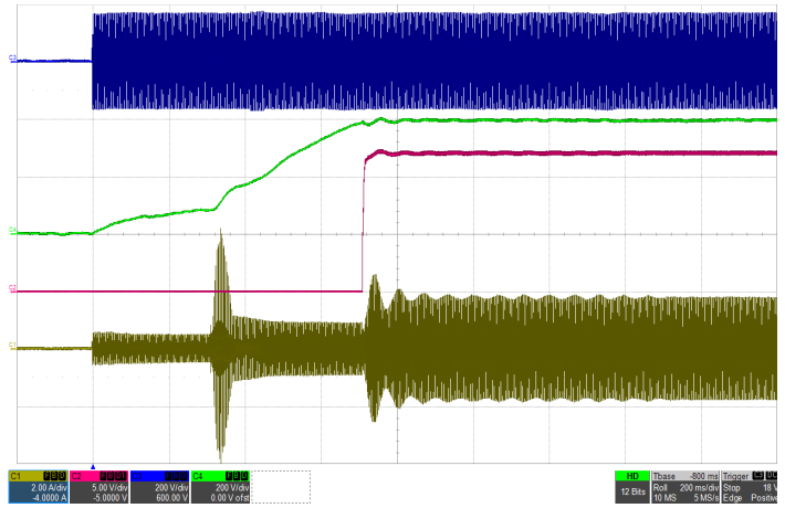
Figure 14: Typical startup waveform with 200µF hold-up capacitor (115Vrms, 400Hz) Top: Vin (200V/div), Top Middle: Hold-up capacitor voltage (200V/div), Bottom Middle: Vout (5V/div), Bottom: In (2A/div), Timebase: (200ms/div).
