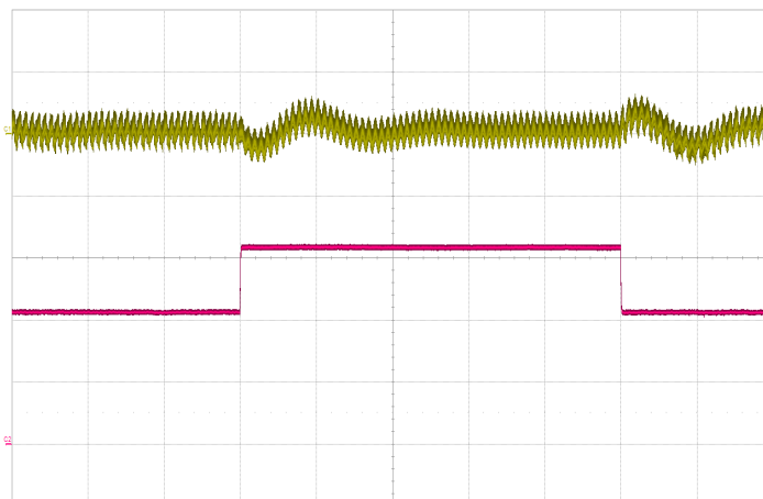
Figure 11: Regulated model output voltage response to step-change in load current with 200µF hold-up capacitor (50%-75%-50% of Iout(max), 115Vrms, 60Hz) Top: Vout (500mV/div), Bottom: Iout (2A/div), Timebase: (100ms/div).
