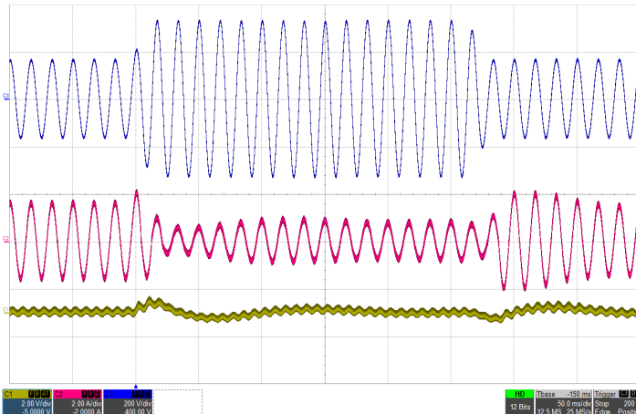
Figure 15: Input voltage transient response with 200µF hold-up capacitor at full load current (115Vrms-230Vrms-115Vrms, 60Hz), Top: Vin (200V/div), Mid: In (2A/div), Bottom: Vout (2V/div), Timebase: (50ms/div).
